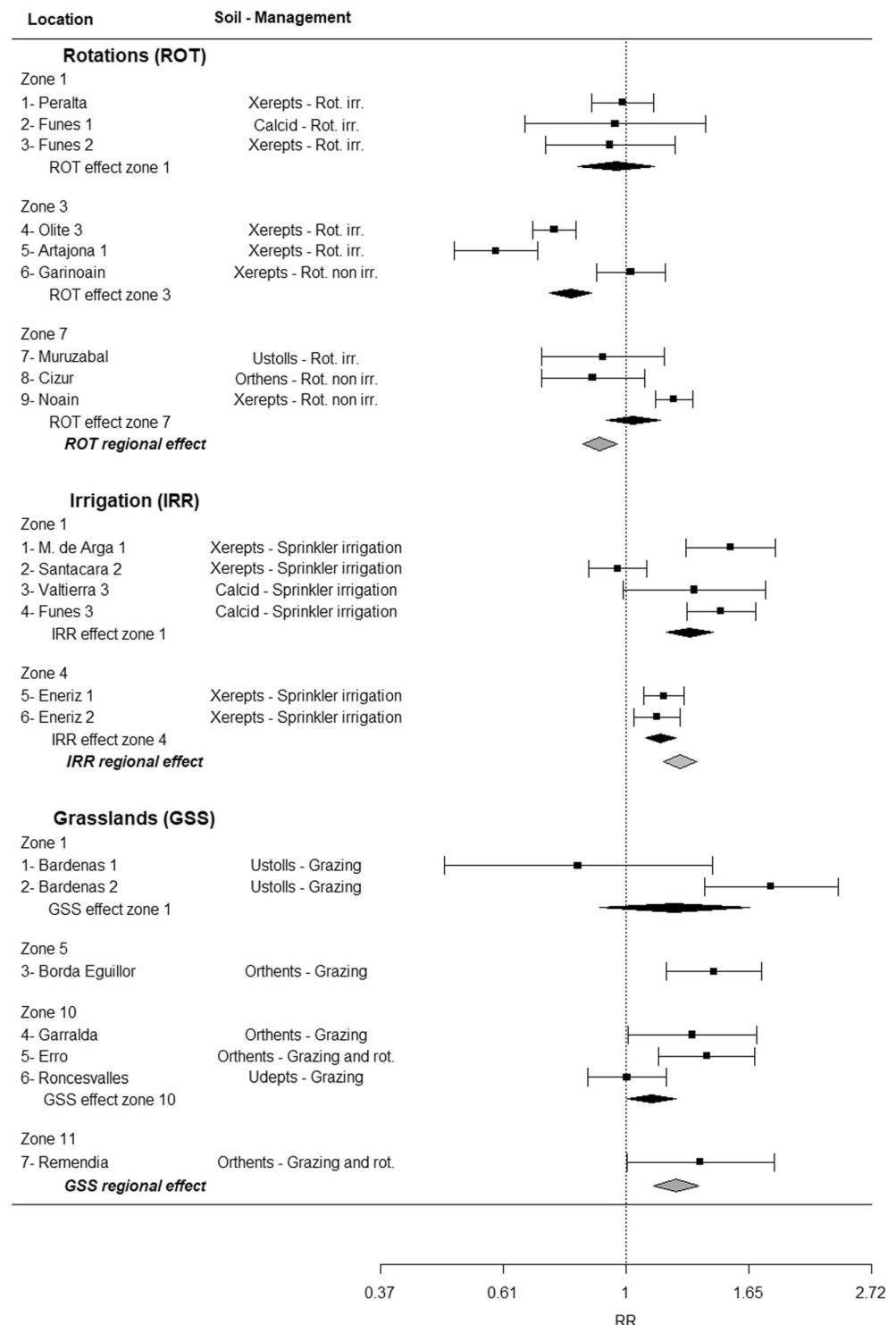
Fig. 3 Response ratio (RR) of soil organic carbon (SOC) stocks (0–20 cm) for adaptive management strategies (rotations ( ROT ), irrigation ( IRR ), and controlled grazing and/or rotation in grasslands ( GSS )). Zones correspond to those in Fig. 1. The effect was considered significant when the 95% confidence interval (CI) of the RR did not overlap one ( \alpha = 0.05 )
