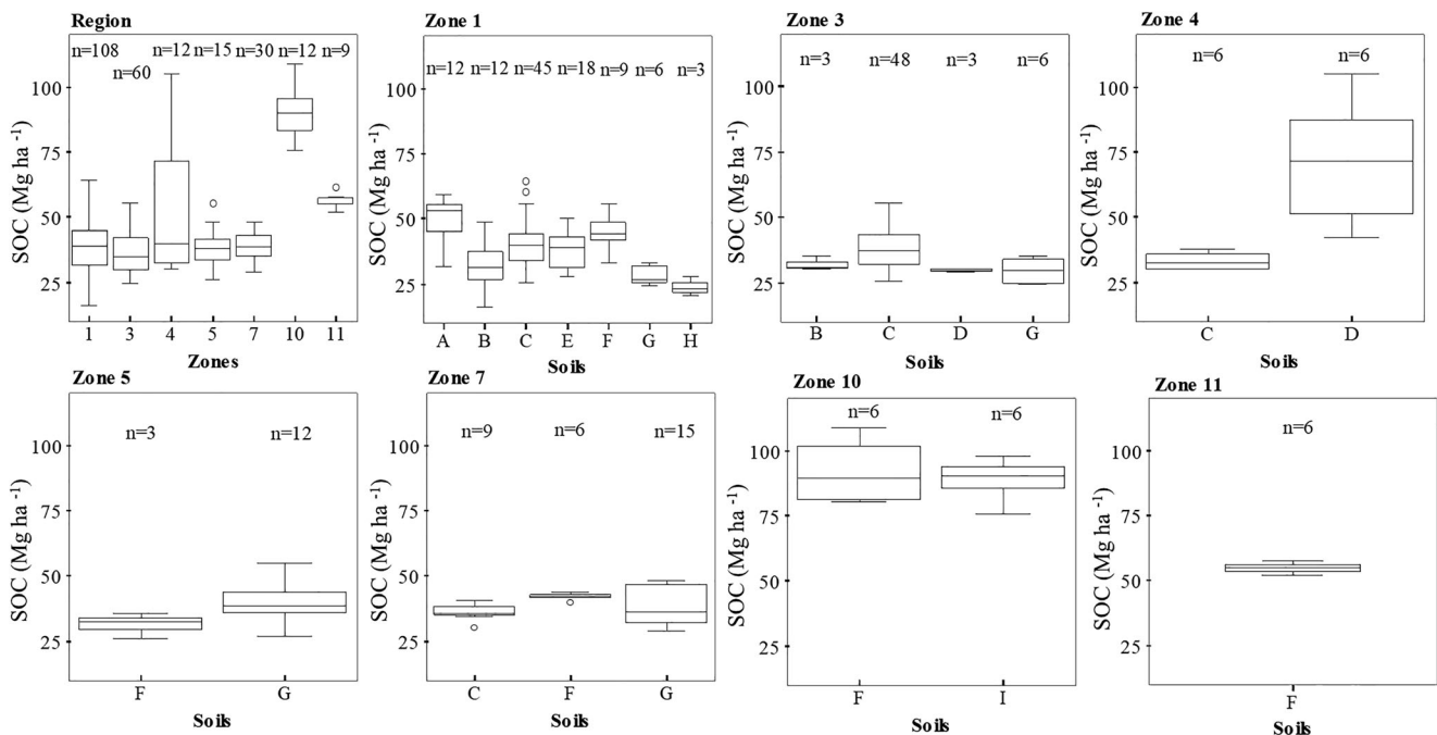
Fig. 2 Soil organic carbon (SOC) stocks in conventionally managed topsoils (0–20 cm) in the region and in the zones selected for this study, for the different type of soils in each zone. A Xerolls, B Ustolls, C Xerepts, D
