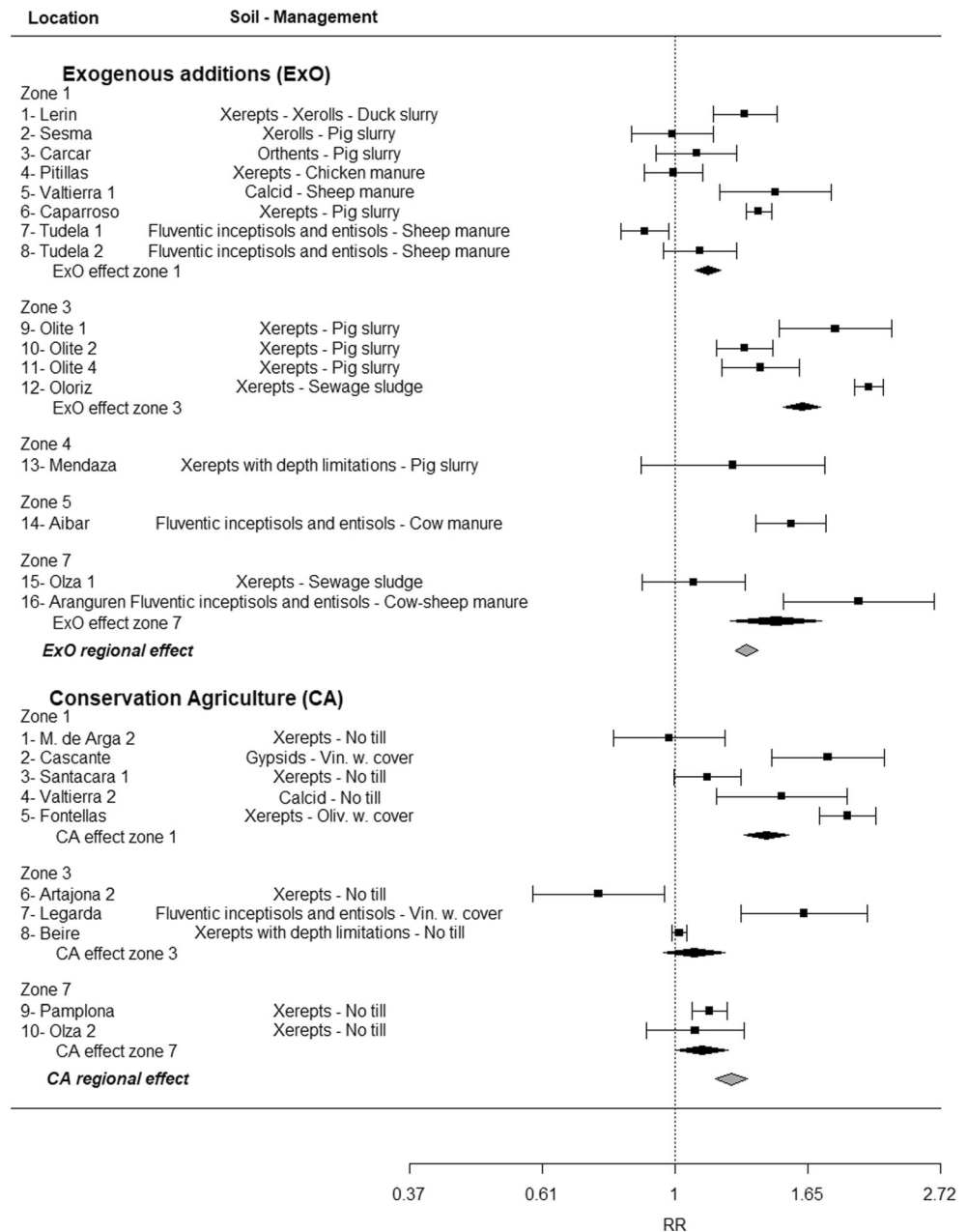
Fig. 4 Response ratio ( RR ) of soil organic carbon ( SOC ) stocks (0–20 cm) for adaptive management strategies (addition of exogenous sources of organic C ( ExO ) and conservation agriculture ( CA )). Zones correspond to those in Fig. 1. The effect was considered significant when the 95% confidence interval ( CI ) of the RR did not overlap one ( \alpha = 0.05 )
